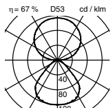
Freestanding uplighter, CLD Controlled Luminance Diffusor
