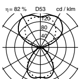
Wall mounted luminaire, CLD Controlled Luminance Diffusor
