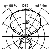
Freestanding uplighter, CLD Controlled Luminance Diffusor
